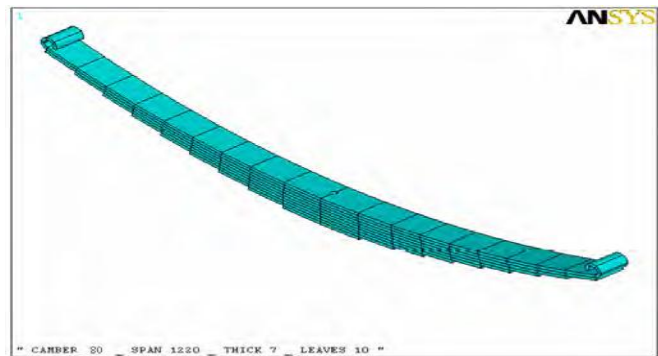
Full model of leaf spring
