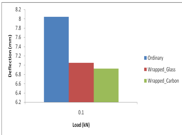
Graph No 5.14 :Comparative Study of Load Ordinary ,CF-Specimen & GF-Specimen
