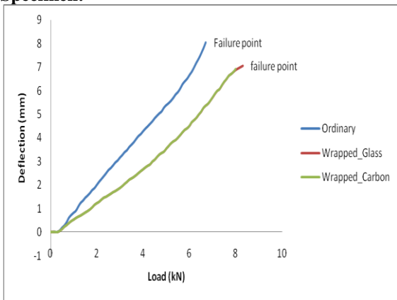
Graph No 5.13 :Comparative Study of Load Ordinary ,CF-Specimen & GF-Specimen
